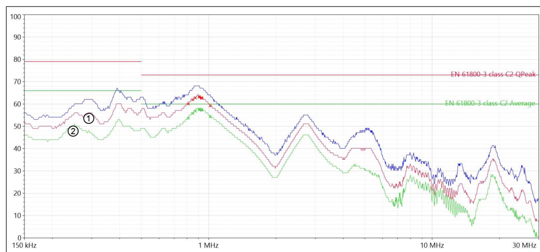
Fig. 11: 30E6T60-1150 Interference voltage measurement C2
