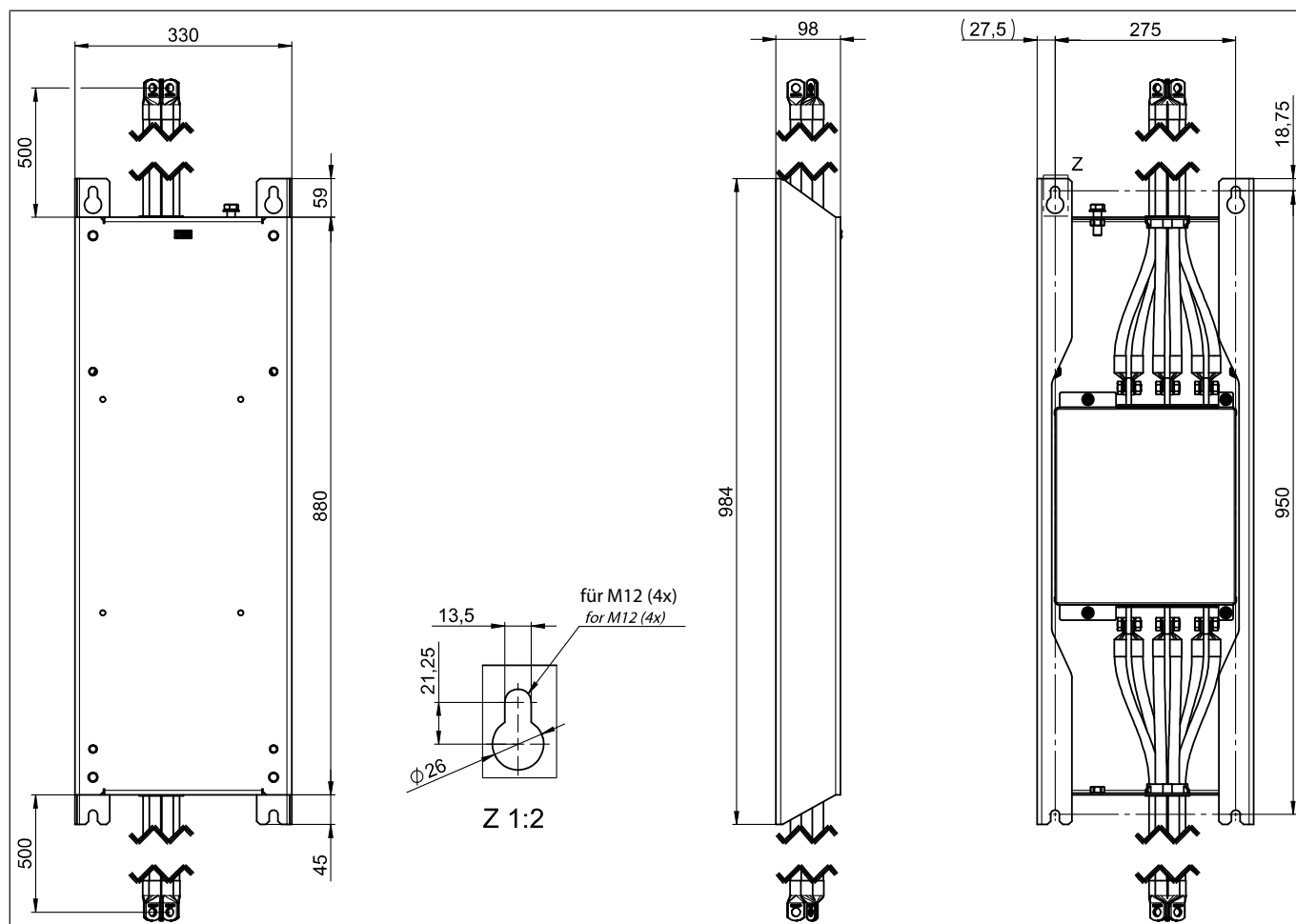
Fig. 7: Dimensions 28...30E6T60-1150
