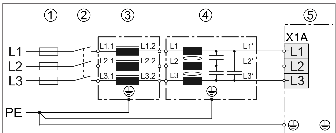
Fig. 8: Connection 3ph choke filter drive controller
