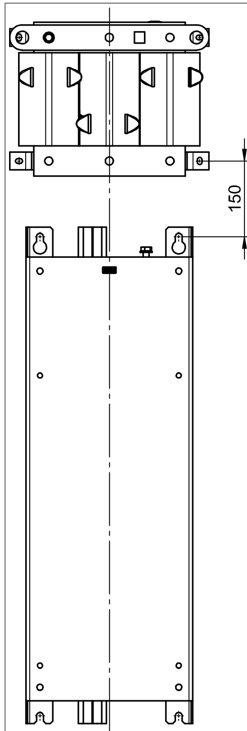
Fig. 6: Installation distance between HF filter and mains choke
