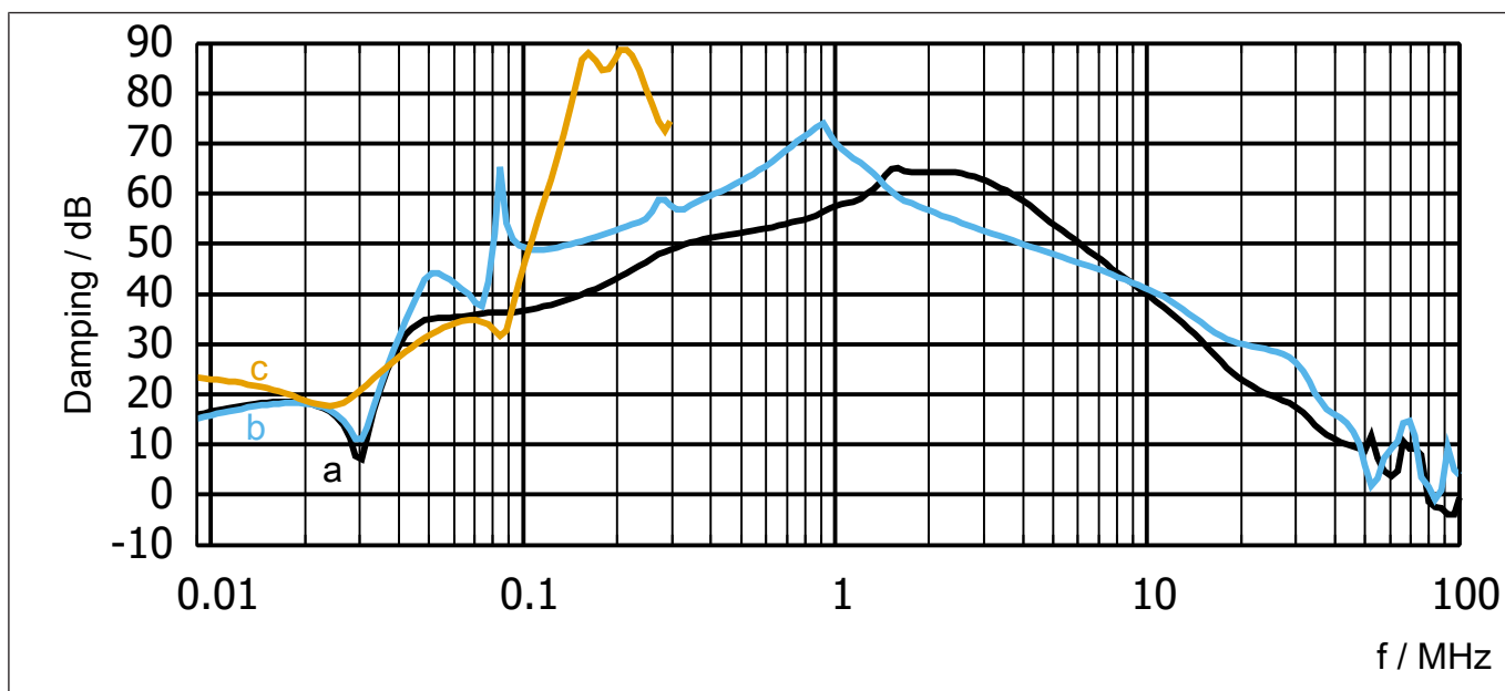
Fig. 2: Insertion loss 28E6T60-1150
