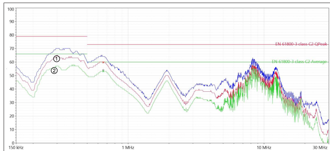
Fig. 10: 28E6T60-1150 Interference voltage measurement C2
