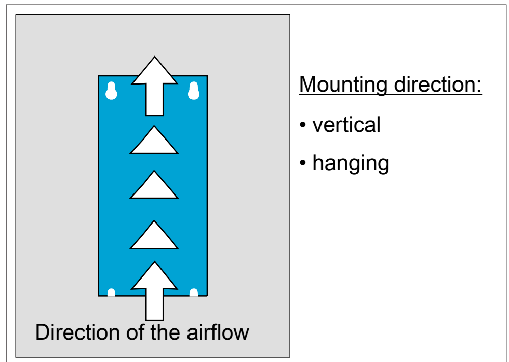
Fig. 4: Permitted mounting orientation
