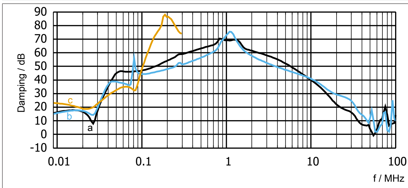
Fig. 3: Insertion loss 30E6T60-1150
