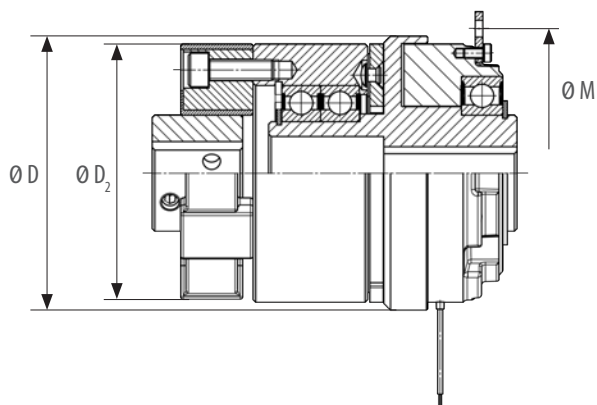
Shaft-mounted (Size 08-12)
