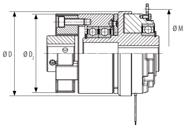
Shaft-mounted (Size 08-12)
