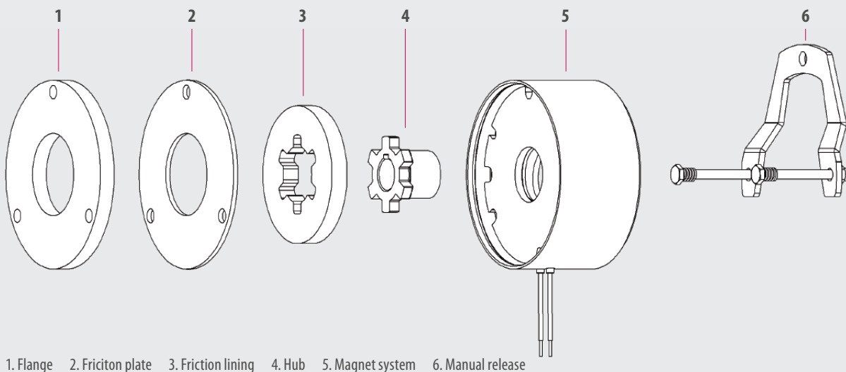
1. Flange 2. Friction plate 3. Friction lining 4. Hub 5. Magnet system 6. Manual release
