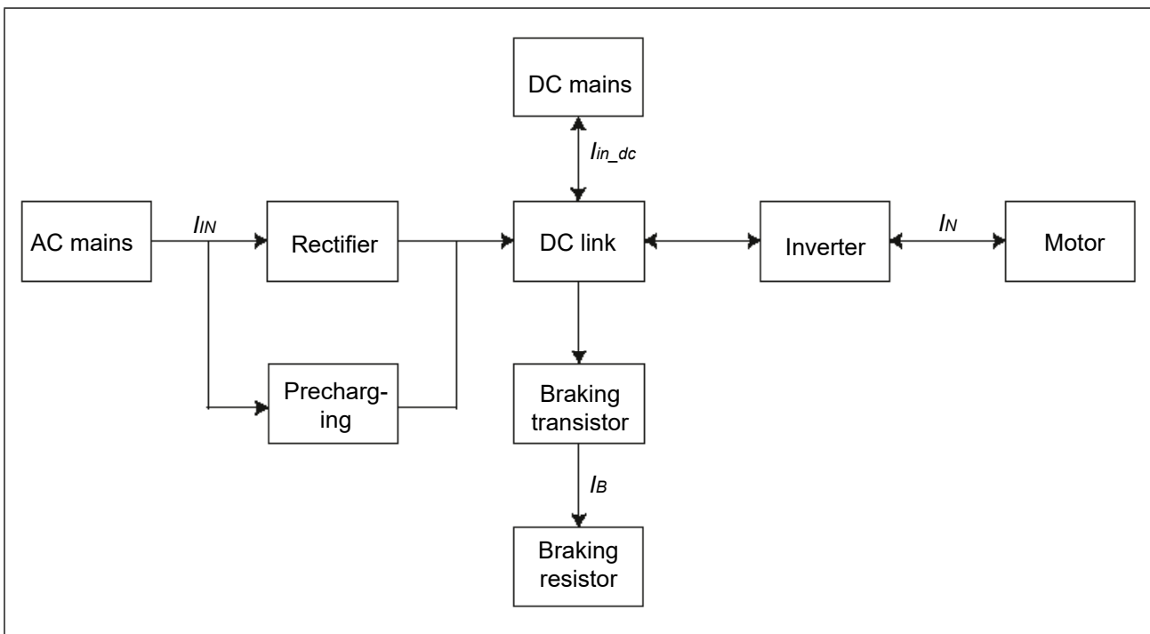
Figure 7: Block diagram of the energy flow
