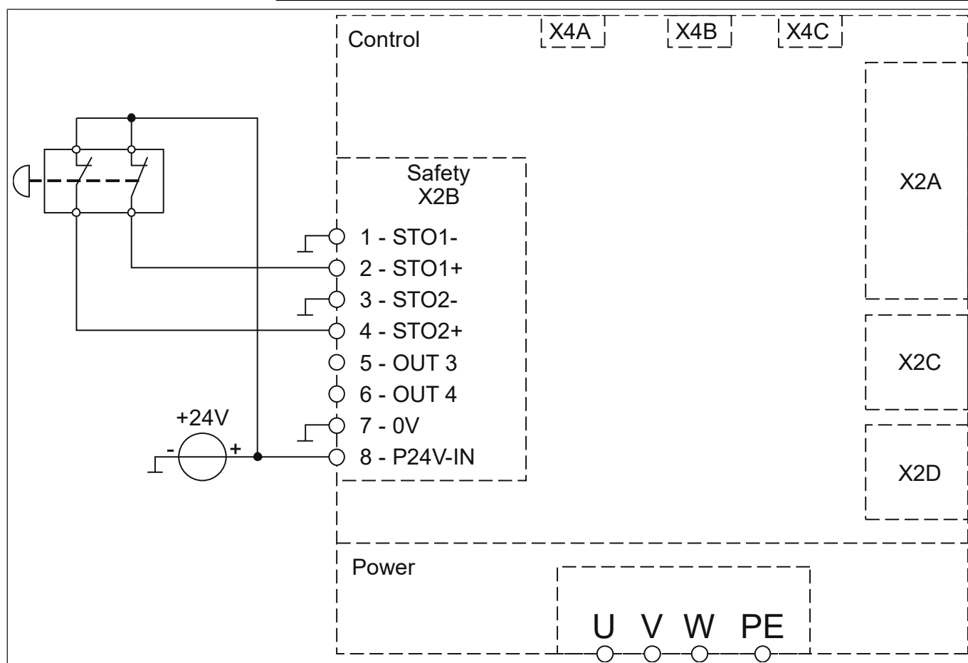
Fig. 9: Direct switch-off with emergency stop switch
