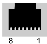
Fig. 9: RJ45 socket front view
