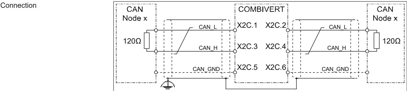
Fig. 3: Connection CAN bus
