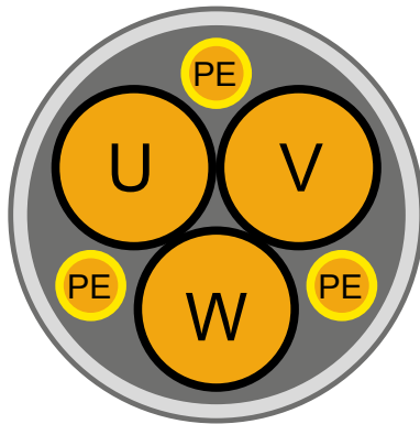
Figure 29: Symmetrical motor line
